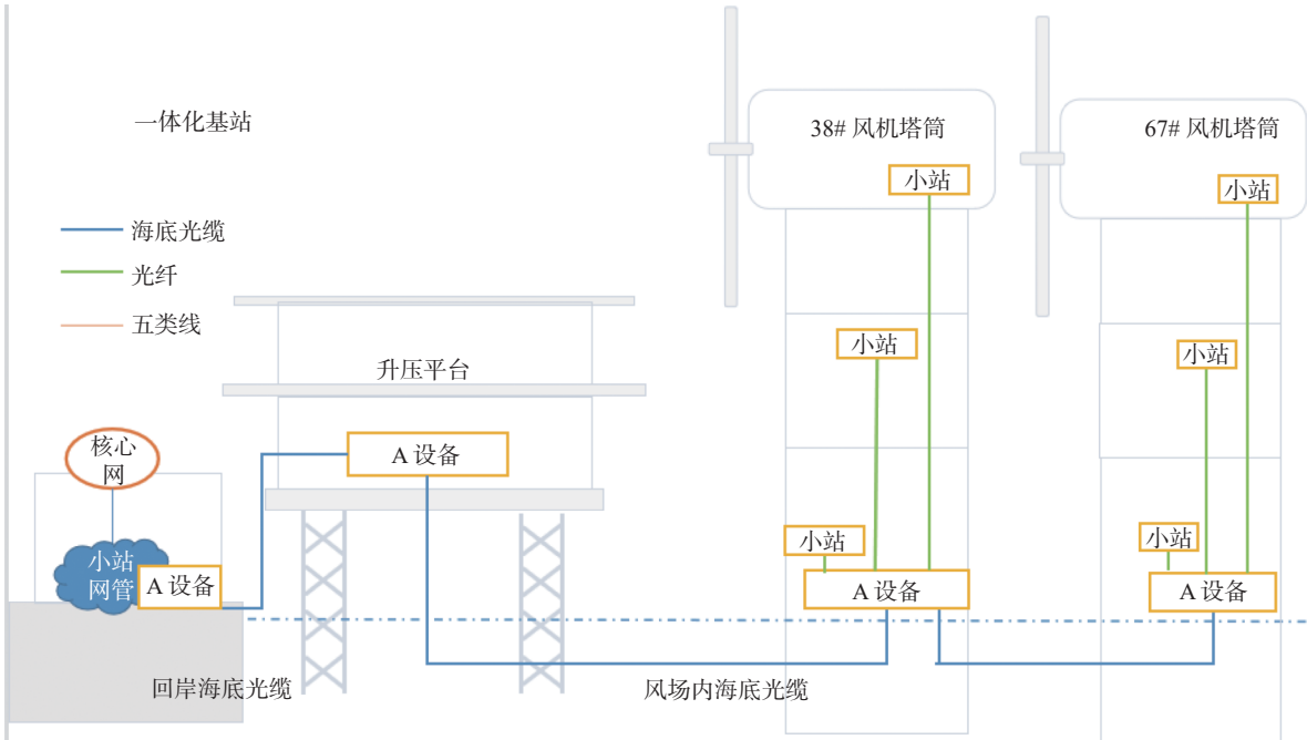
图 7 基于 STN 承载网的一体化小站方案图 Fig. 7 Scheme diagram of integrated small station based on STN bearer network
